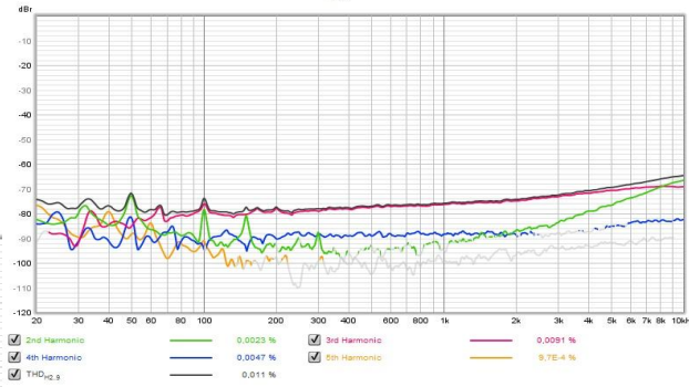
9V @ 2ohm
