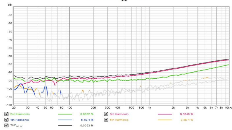
U70%/25V @ 32ohm
