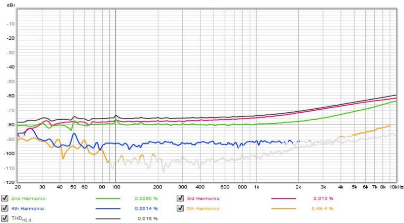
U70%/25V @ 4ohm
